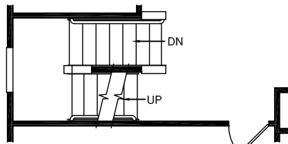
STAIRS ON 2ND FLOOR W/ OPT. ATTIC
