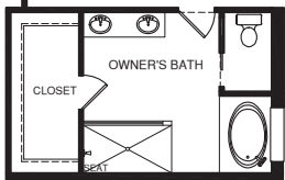
OPT. LUXURY OWNER'S BATH W/ BONUS ROOM
