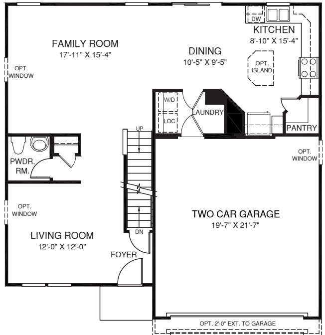
MAIN LEVEL
