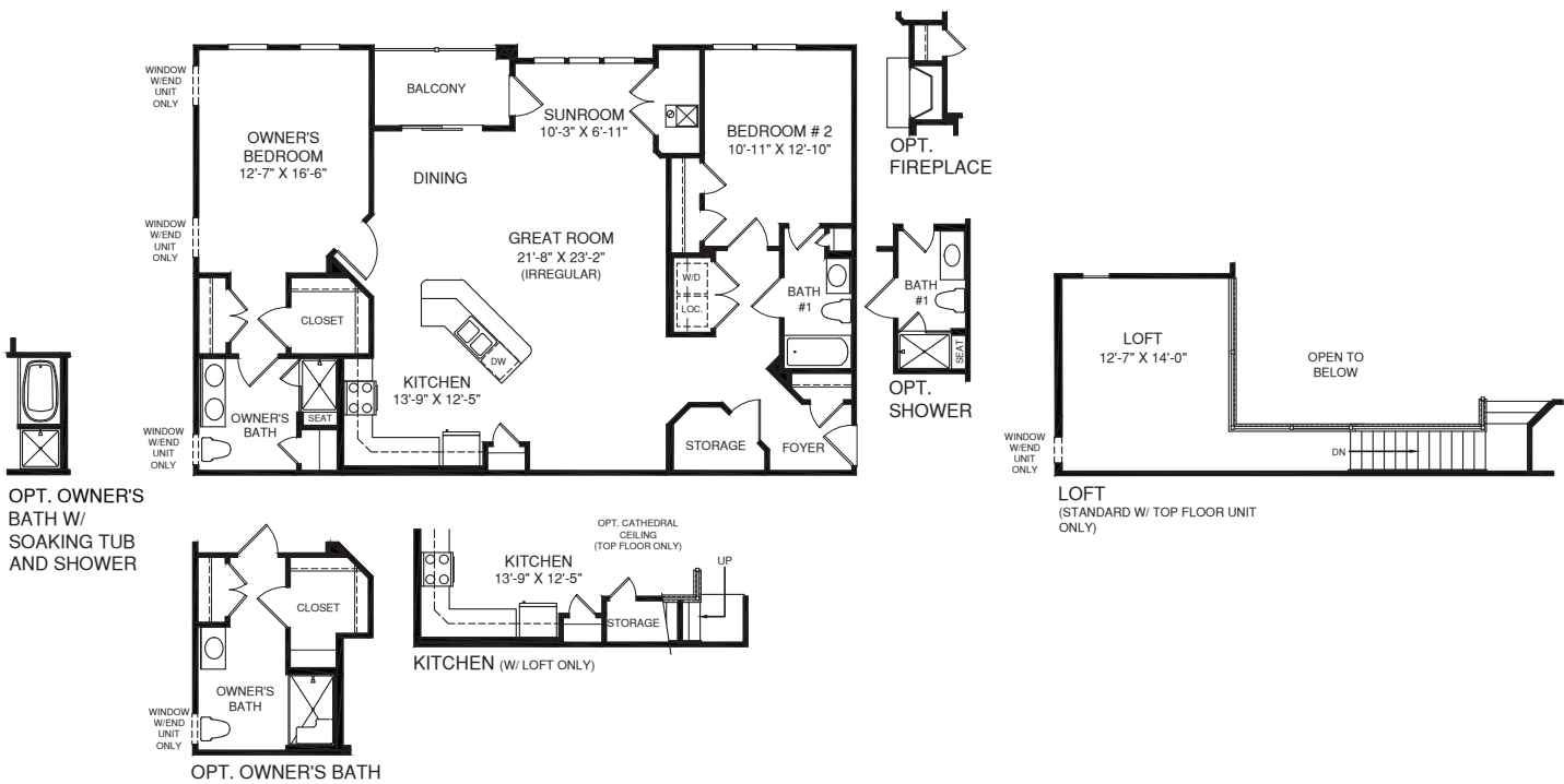
REAR UNIT
