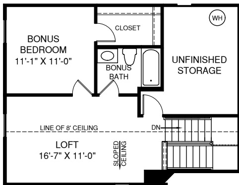
OPT. SECOND FLOOR W/ OPT. BONUS BEDROOM
