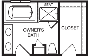
OPT. OWNER'S BATH W/ SOAKING TUB & SHOWER
