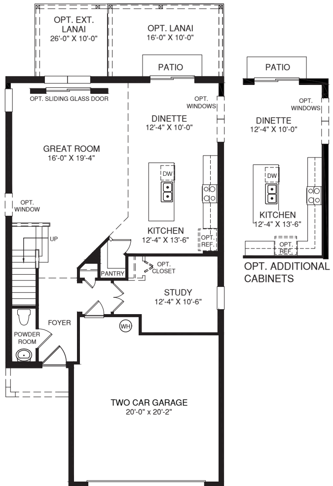
MAIN LEVEL
