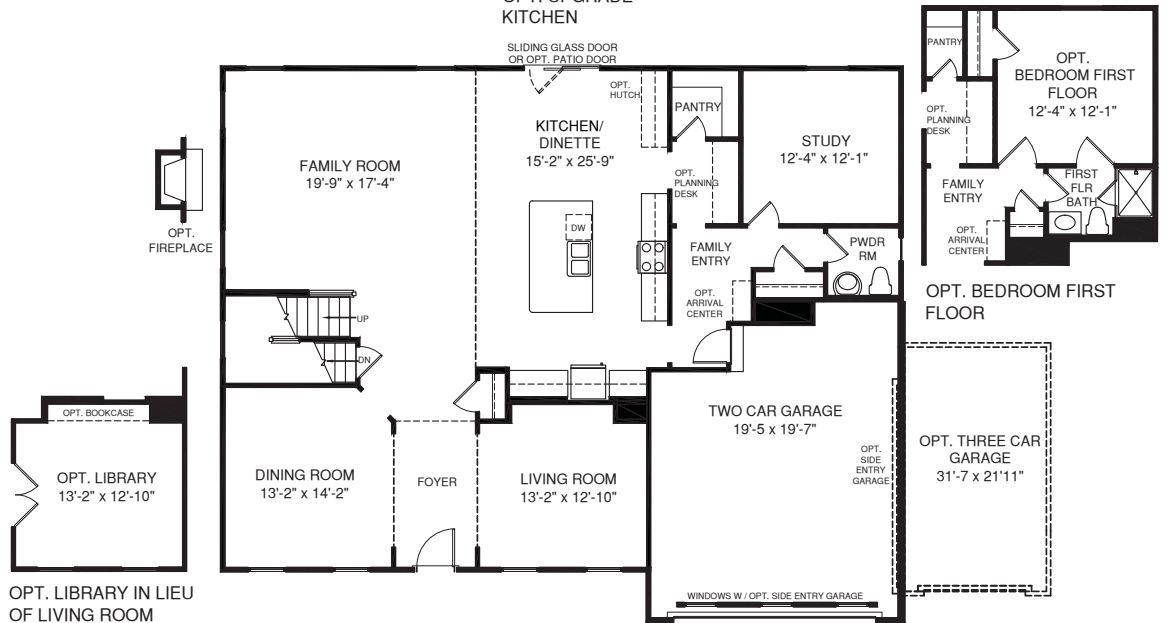
MAIN LEVEL
