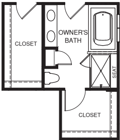
OPT. OWNER'S BATH W/ SOAKING TUB & SHOWER
