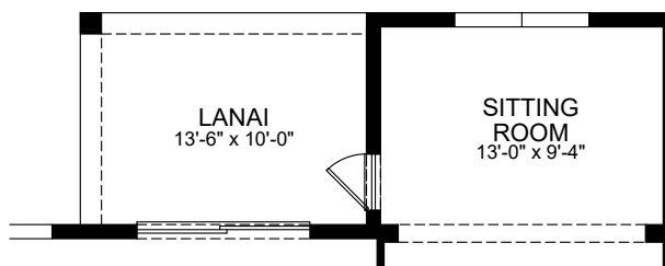
OPT. SITTING ROOM WITH EXTENDED LANAI
