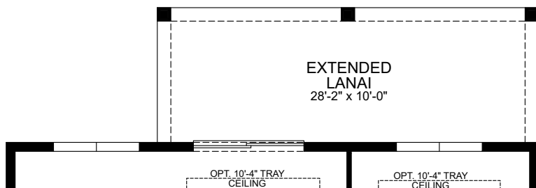
OPT. EXTENDED LANAI
