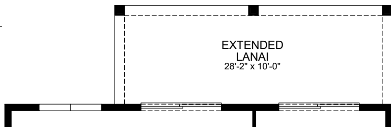
OPT. EXTENDED LANAI WITH OWNERS SUITE SLIDING GLASS DOOR
