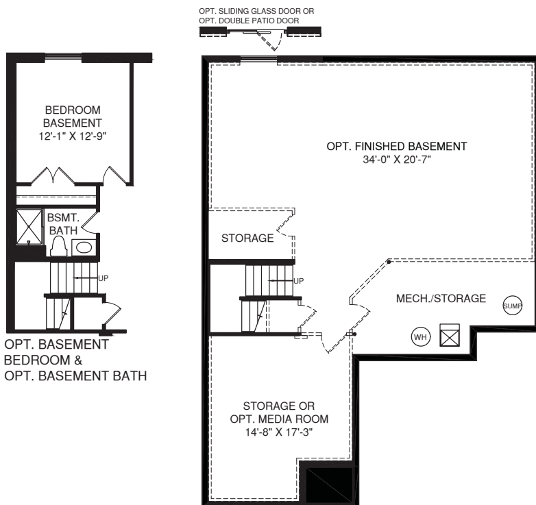
LOWER LEVEL
