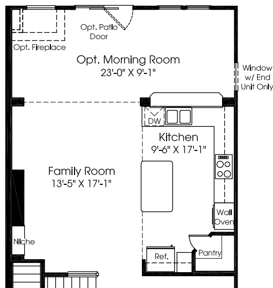
Opt. Morning Room w/ Opt. Appliance Layout
