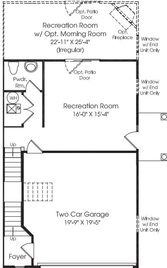
Opt. Side Entry
