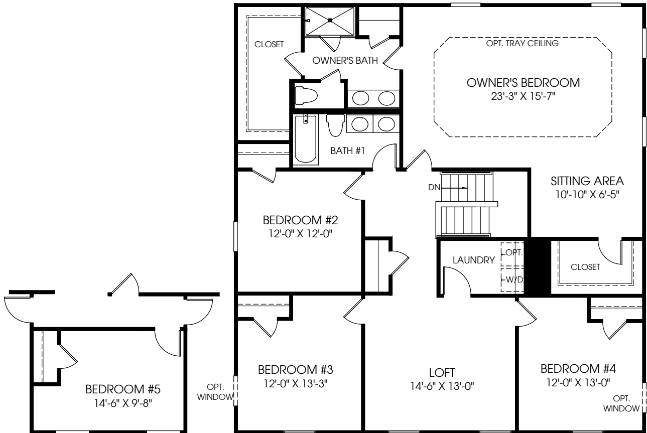
OPT. BEDROOM #5
