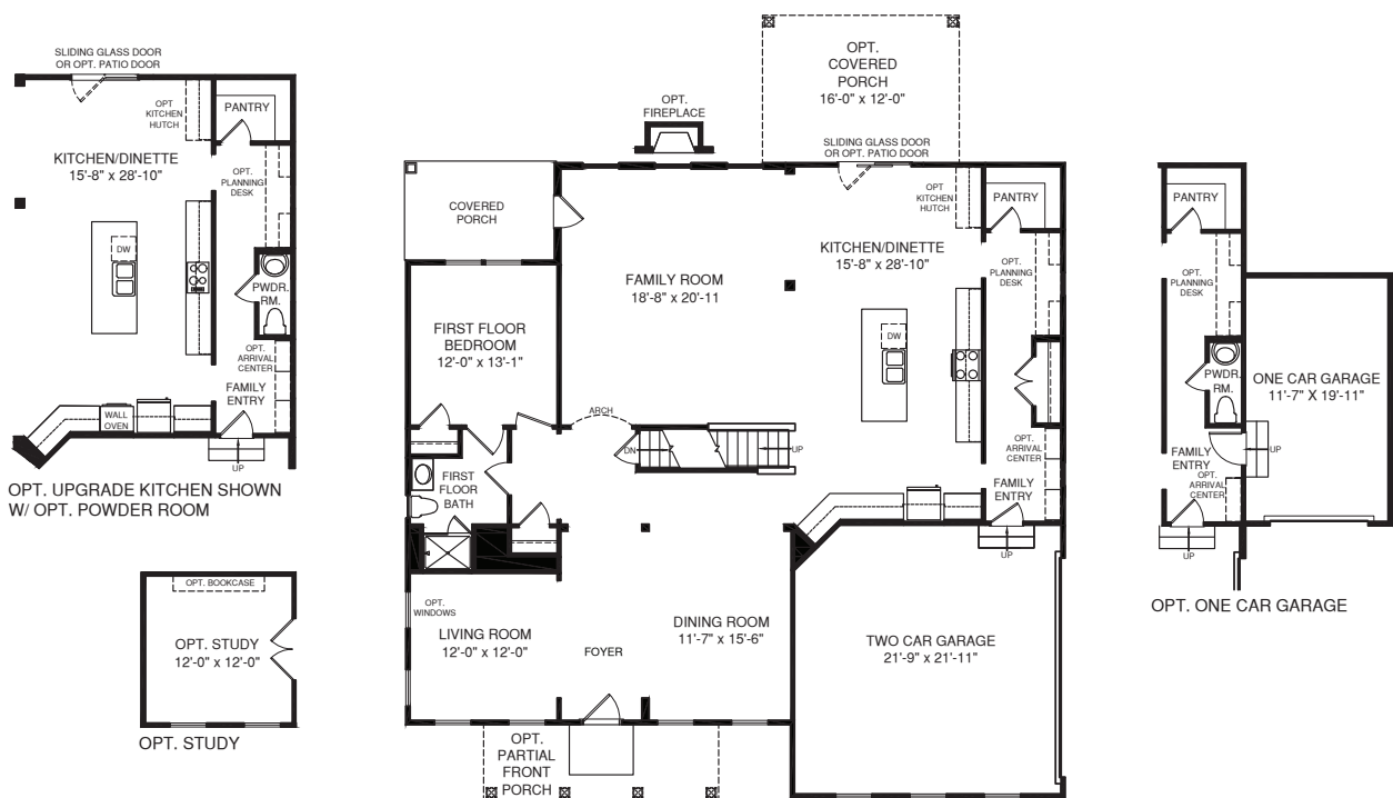
MAIN LEVEL
