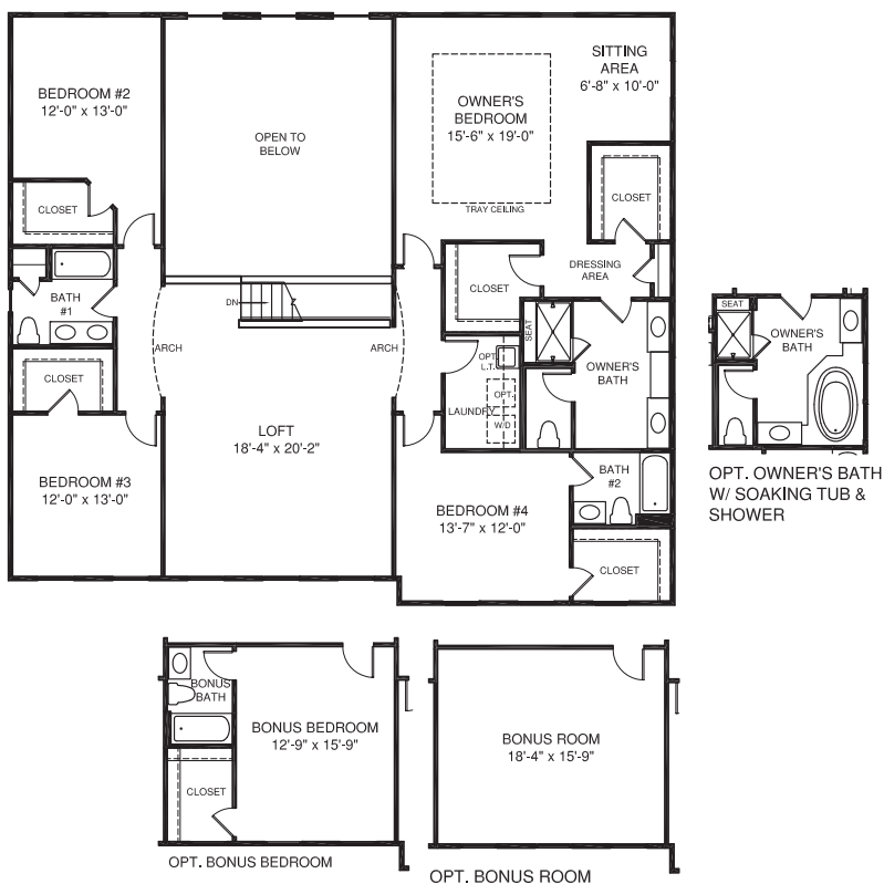
UPPER LEVEL
