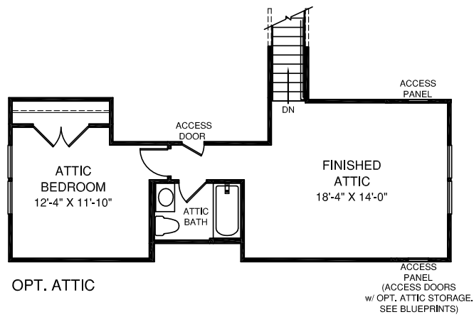
STAIRS W/ OPT. ATTIC
