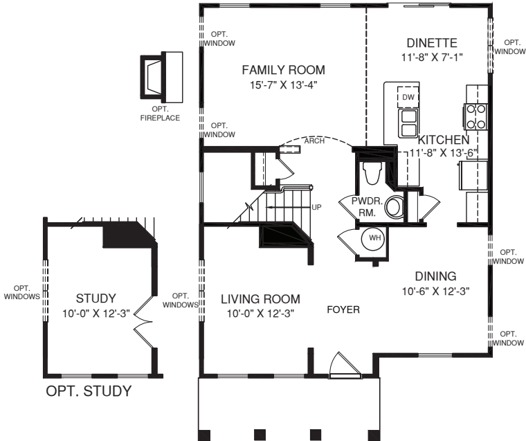
MAIN LEVEL
