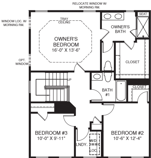
UPPER LEVEL
