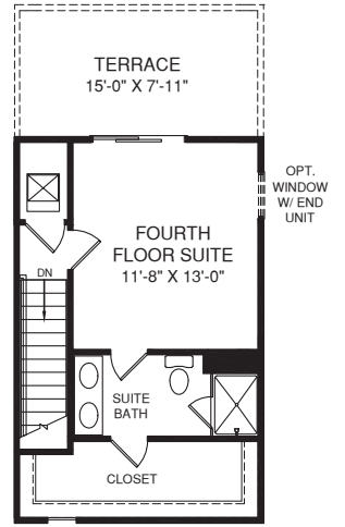
OPTIONAL SUITE FOURTH FLOOR WITH TERRACE
