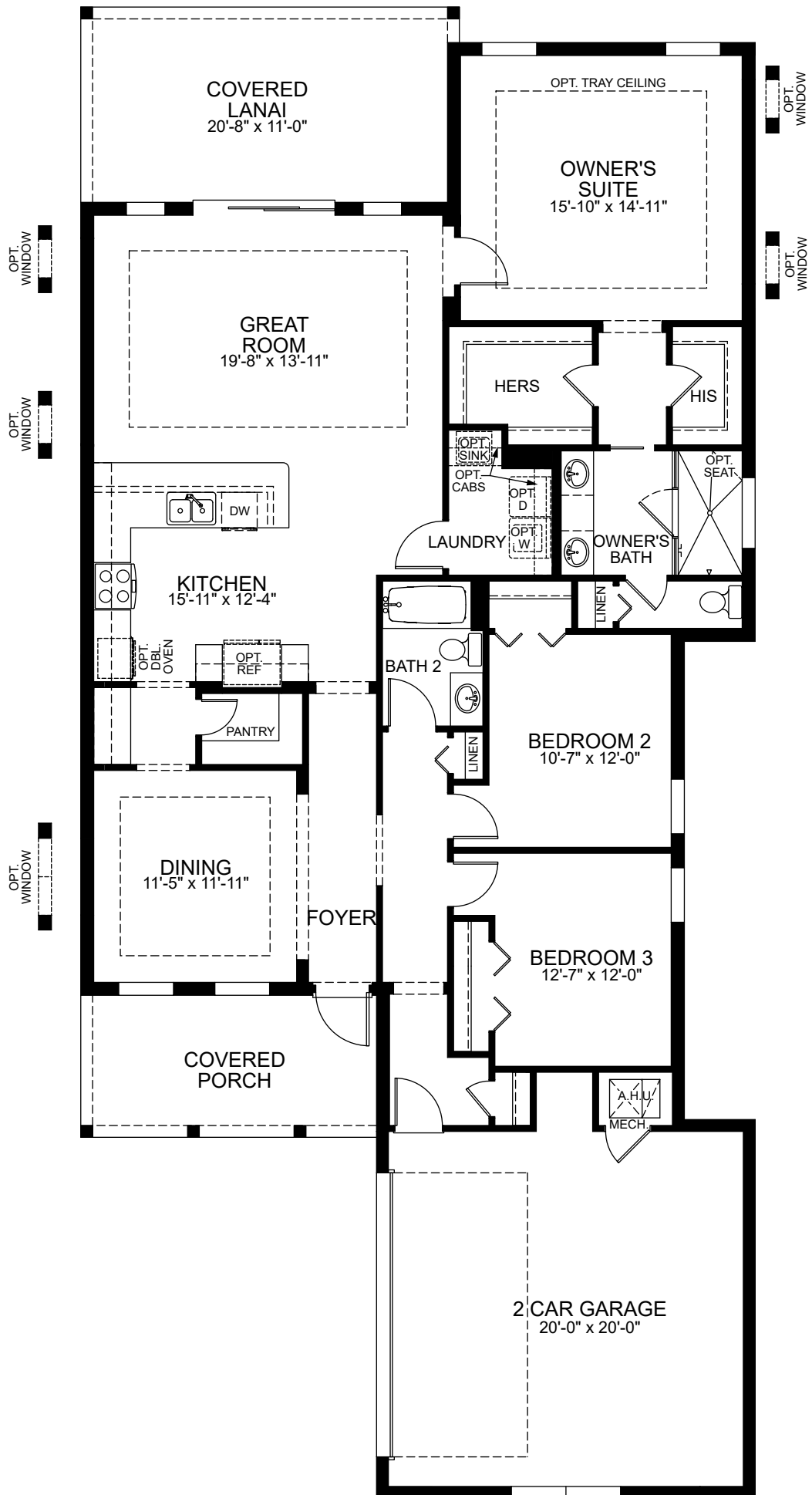
FLOOR PLAN
