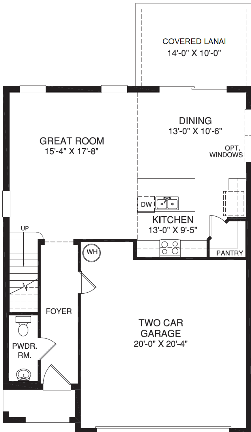
MAIN LEVEL
