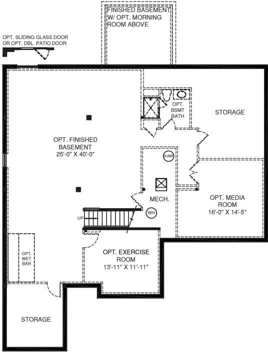
LOWER LEVEL
