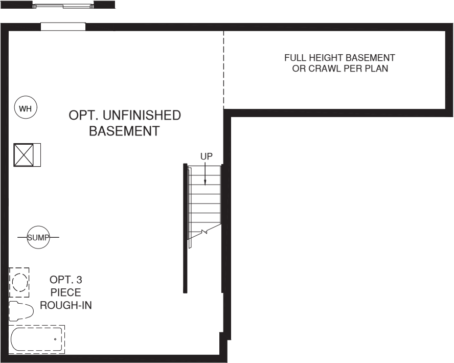
OPTIONAL UNFINISHED BASEMENT
