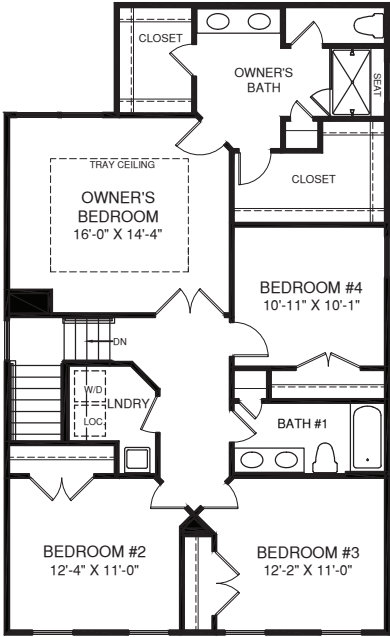
UPPER LEVEL
