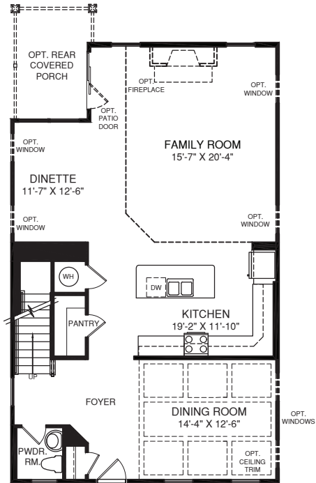
MAIN LEVEL
