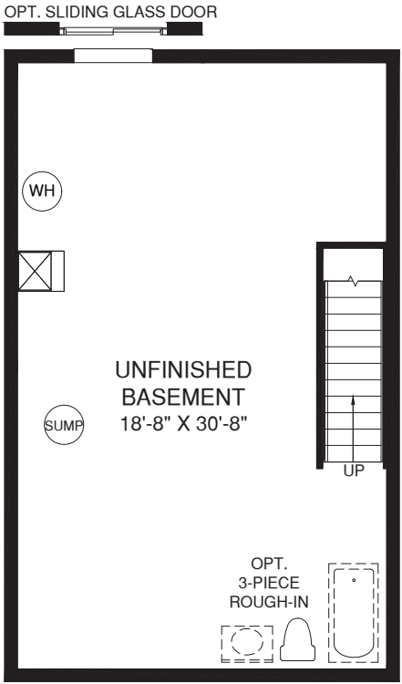
LOWER LEVEL
