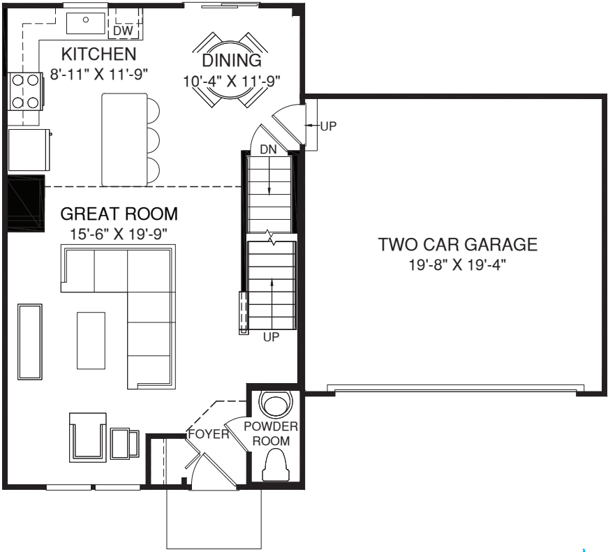
MAIN LEVEL
