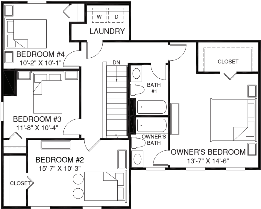
UPPER LEVEL
