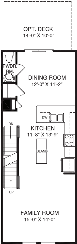
SECOND FLOOR
