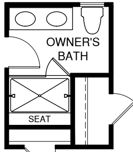
OPT. OWNER'S BATH W/ ROMAN SHOWER
