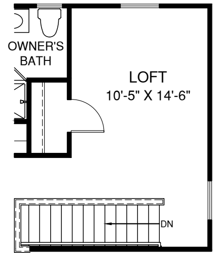
OPT. THREE BEDROOM W/ LOFT
