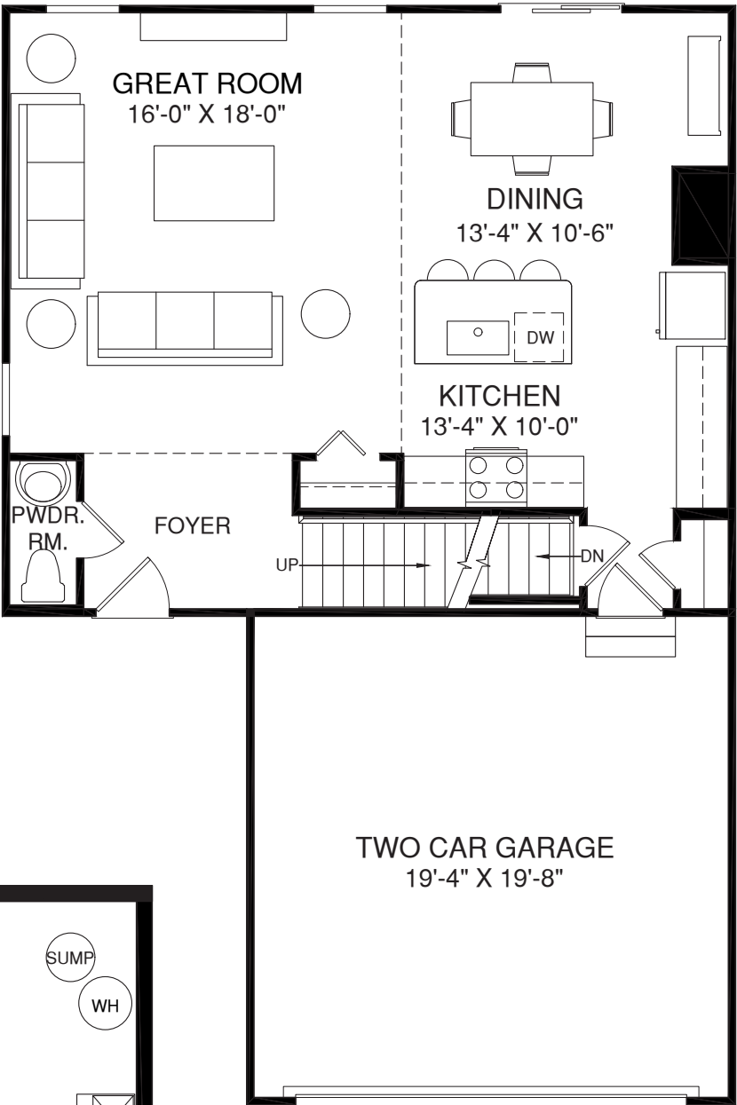
MAIN LEVEL
