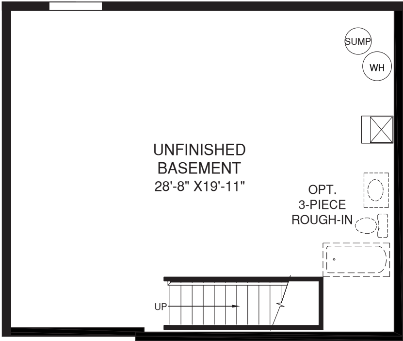
BASEMENT LEVEL
