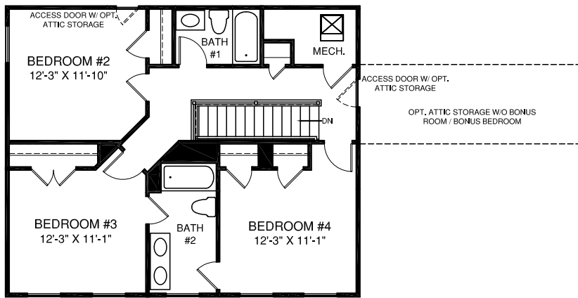
OPT. FOUR BEDROOM W/ BATH #2
