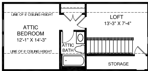
OPT. ATTIC BEDROOM
