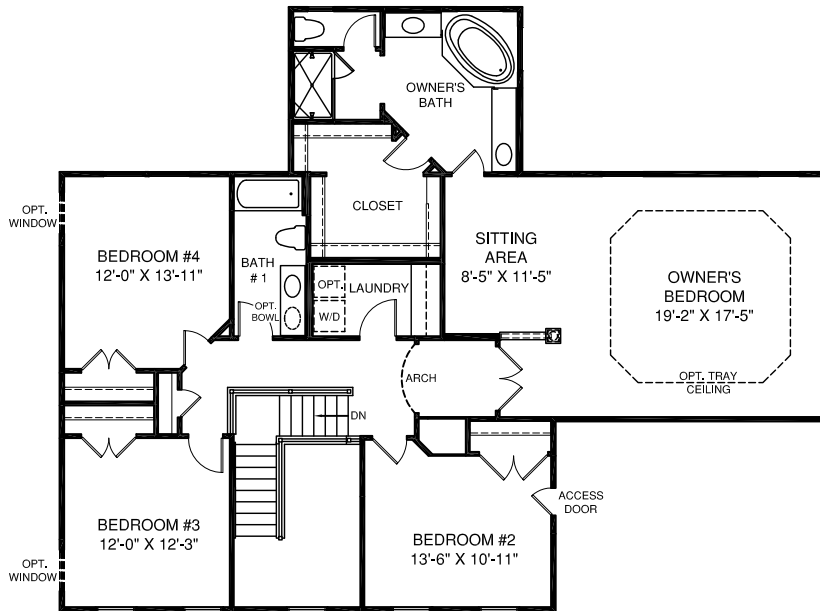
OPT. LUXURY OWNER'S SUITE
