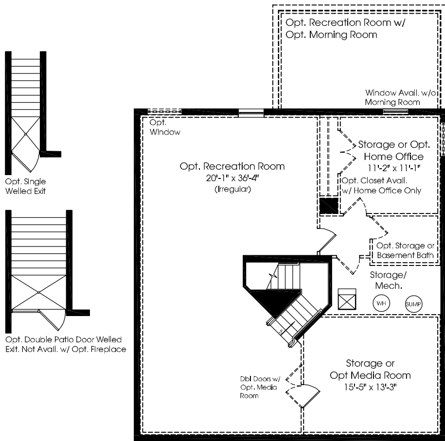
LOWER LEVEL ELEVATION A
