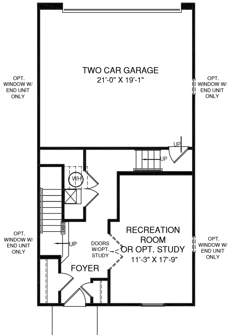
LOWER LEVEL WITH STEP DOWN GARAGE
