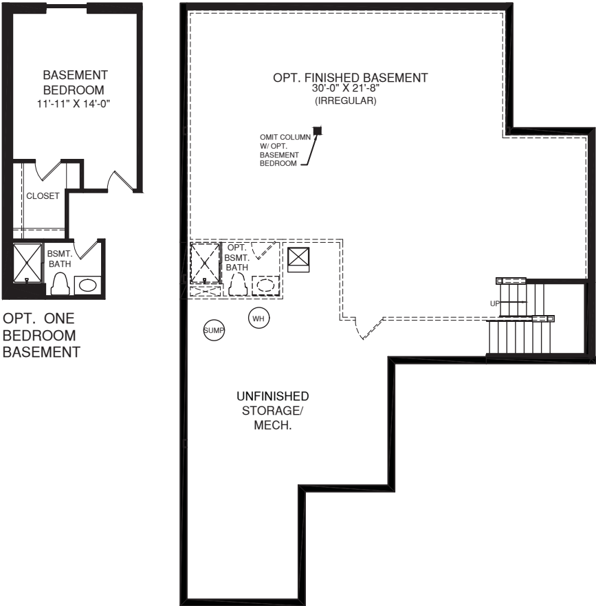
LOWER LEVEL
