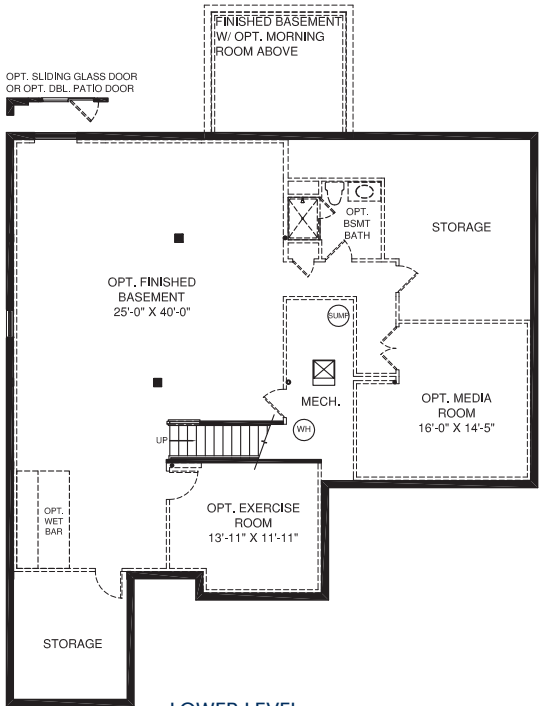
LOWER LEVEL
