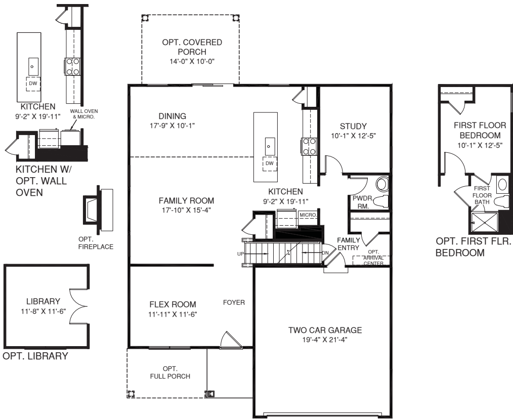
MAIN LEVEL
