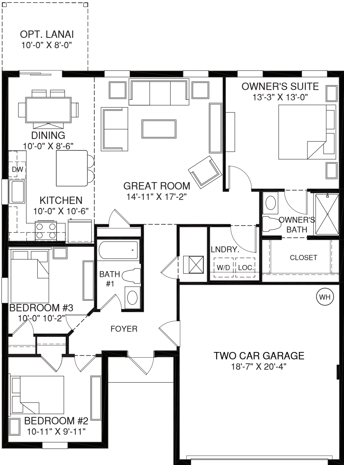
MAIN LEVEL
