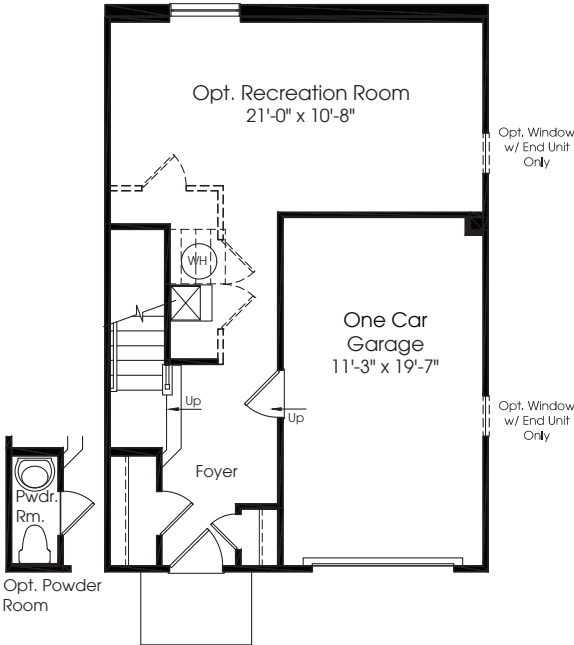
LOWER LEVEL
