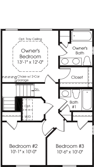
UPPER LEVEL
