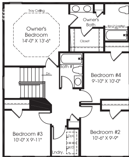
Second Floor W/ Opt. Four Bedrooms
