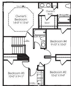
Second Floor W/ Opt. Four Bedrooms
