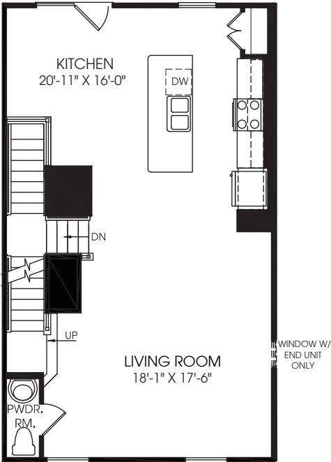
MAIN LEVEL
