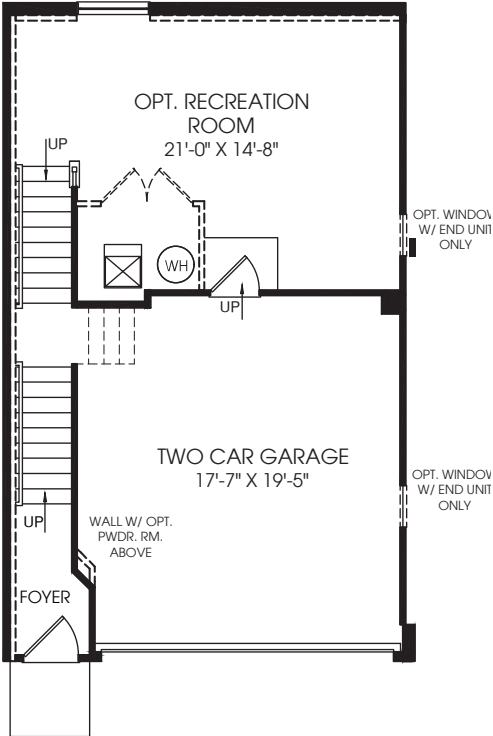
LOWER LEVEL
