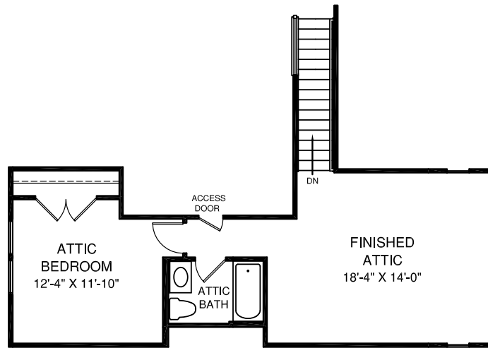
OPT. ATTIC
