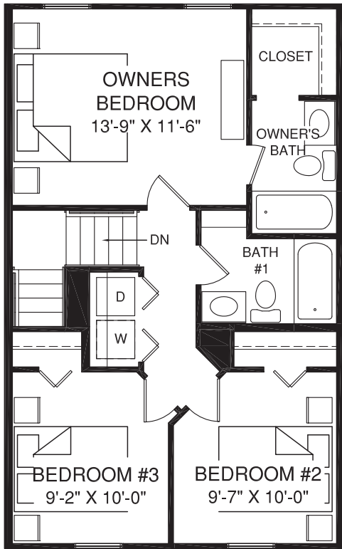
UPPER LEVEL
