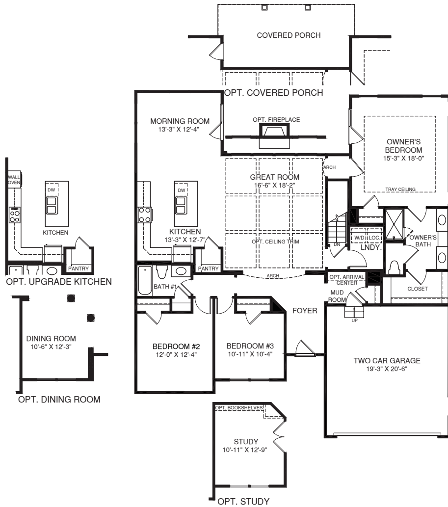
MAIN LEVEL
