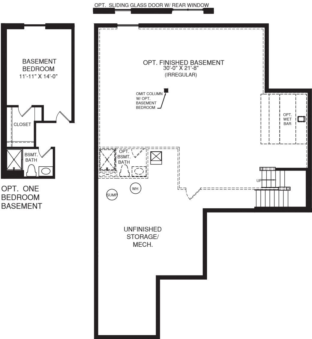
LOWER LEVEL
