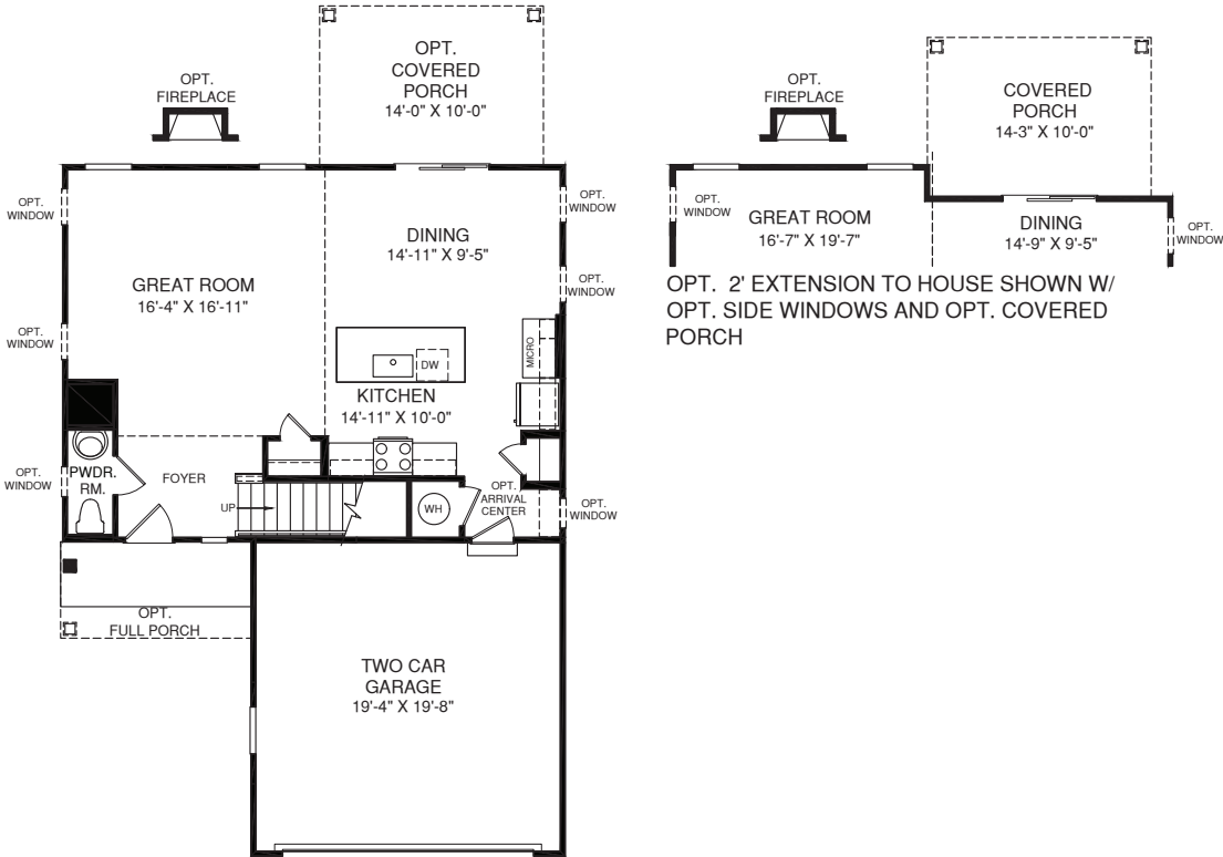
MAIN LEVEL
