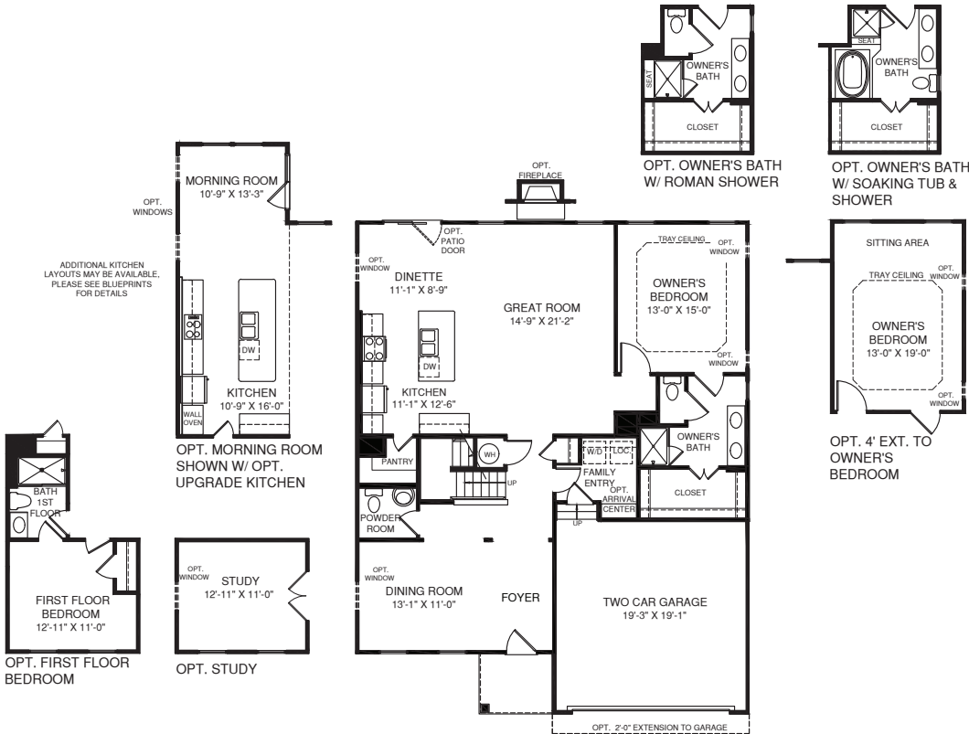
MAIN LEVEL
