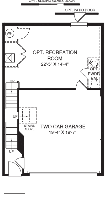
OPT. 4' EXTENSION
