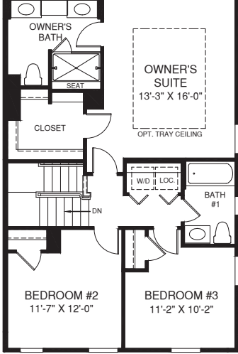
OPT. 4' EXTENSION
