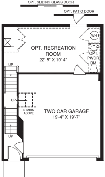
LOWER LEVEL
