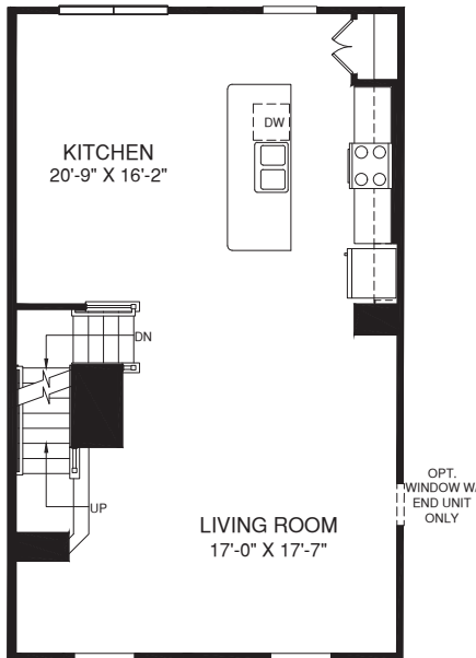
MAIN LEVEL
