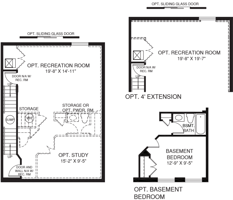
LOWER LEVEL
