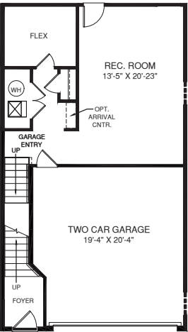
OPT. 4'-0" EXTENSION TO HOUSE
