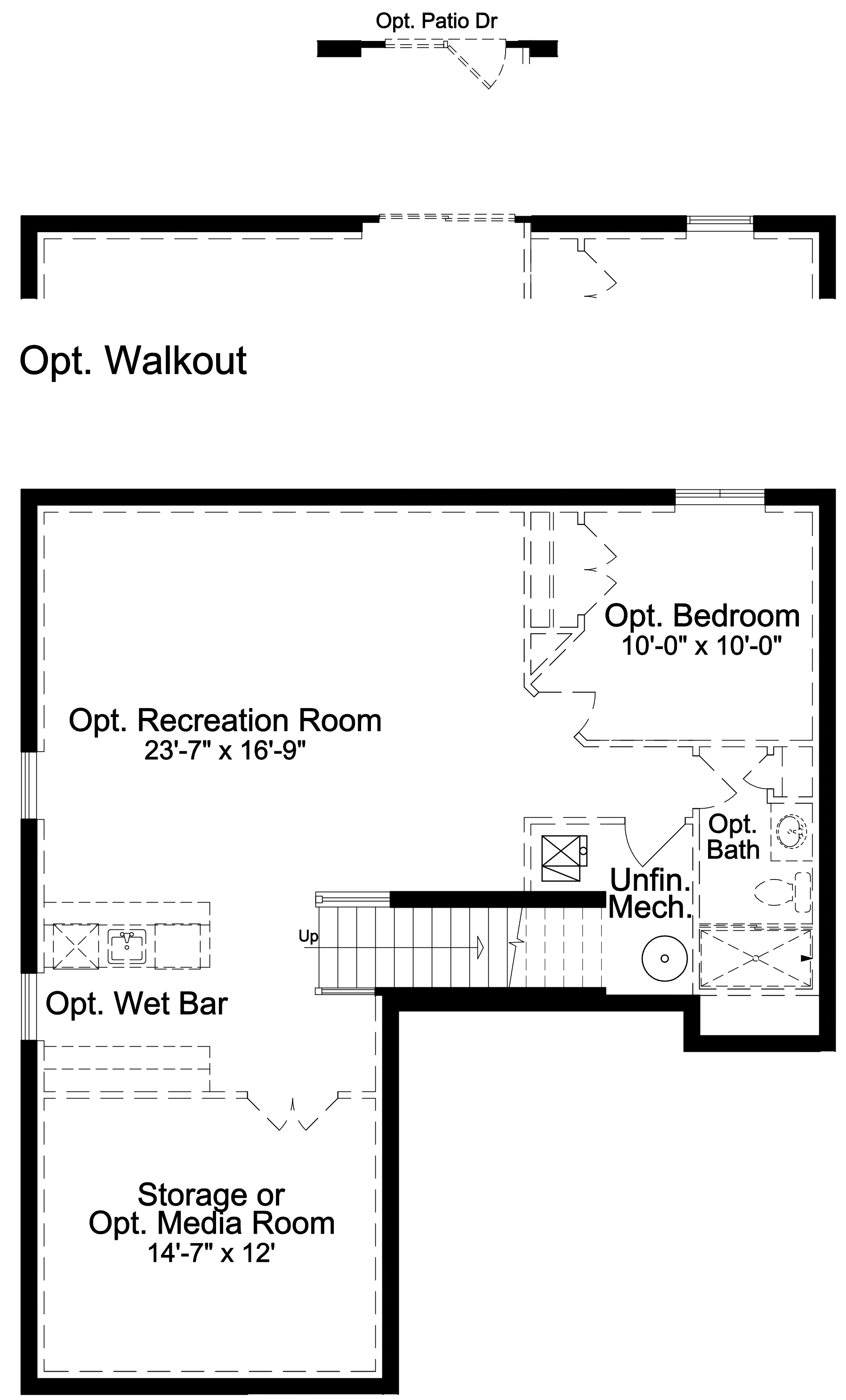
Opt. Finished Basement Plan
