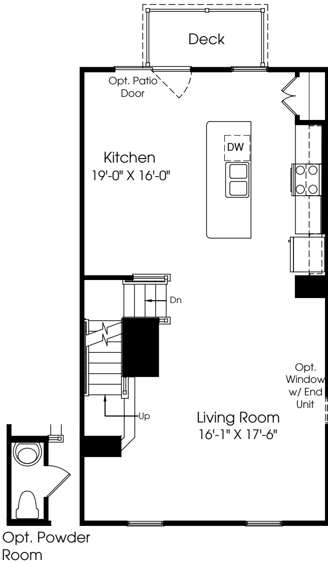
MAIN LEVEL
