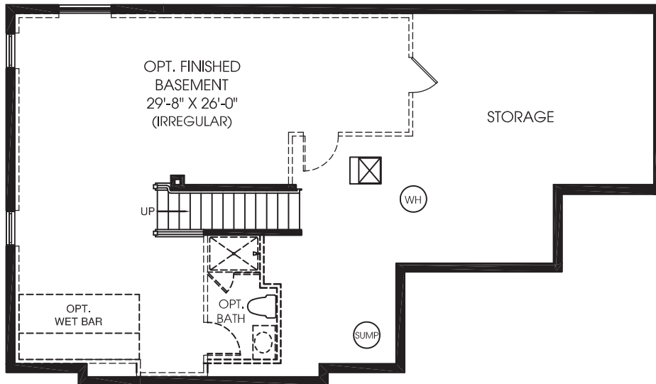
OPT. FINISHED BASEMENT W/ OPT. MORNING ROOM
